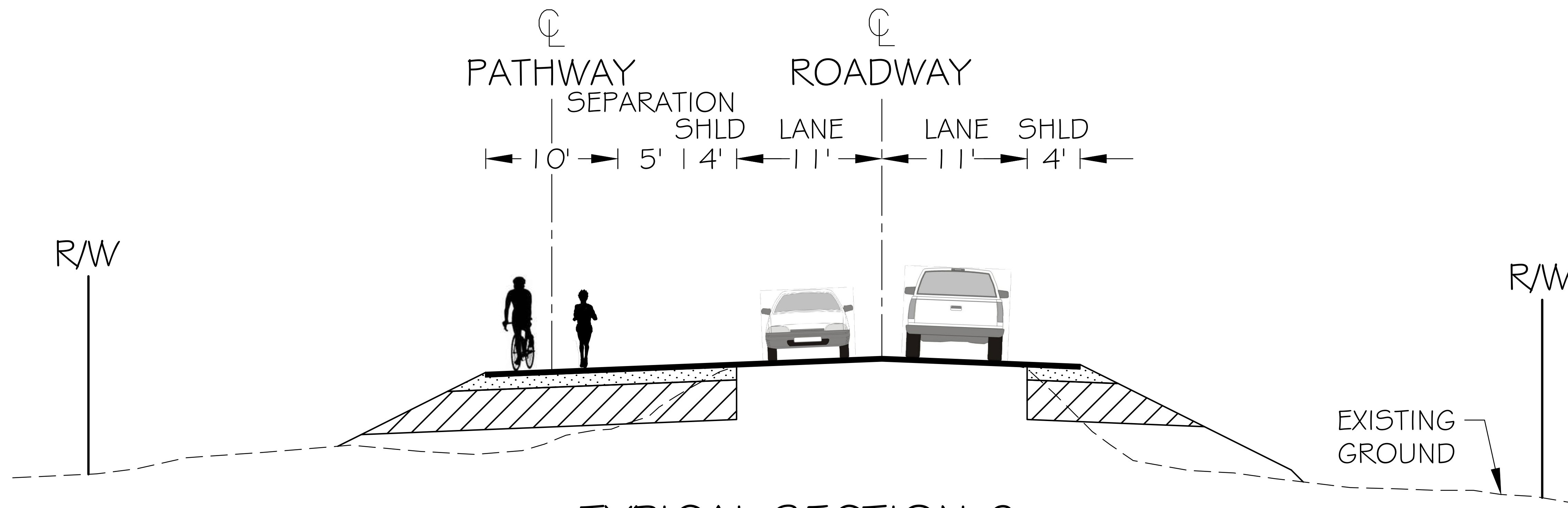
TYPICAL SECTION 2
