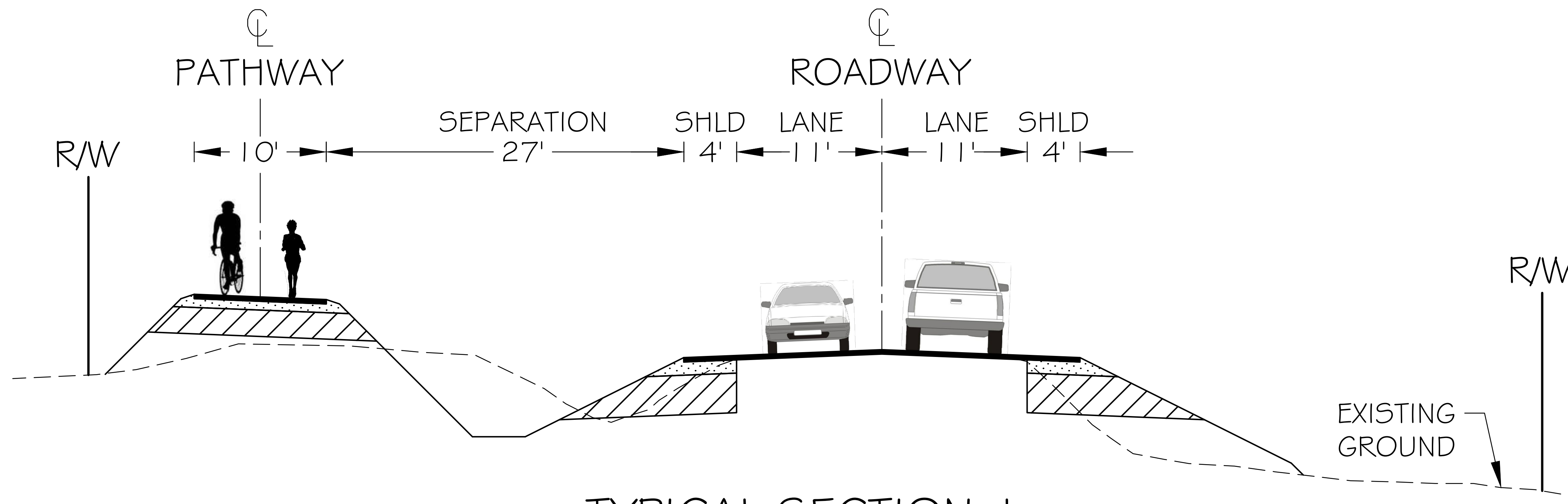
TYPICAL SECTION 1
